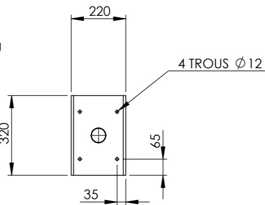
PLATINE INCLINAGLE
